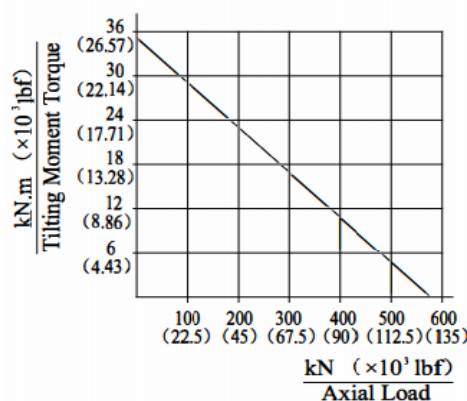
MOMENT LOAD CHART Axial Load & Tilting Moment
