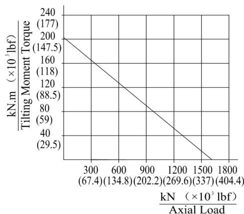
MOMENT LOAD CHART Axial Load & Tilting Moment
