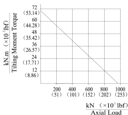
MOMENT LOAD CHART Axial Load & Tilting Moment
